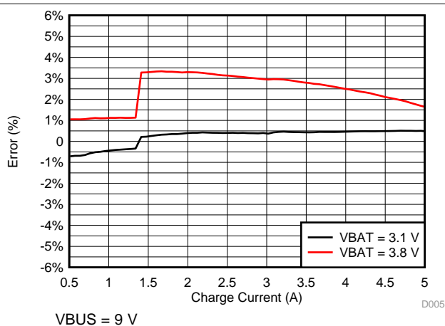
图 4. Charge Current Accuracy vs Charge Current I 2 C Setting
