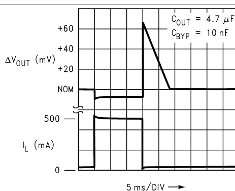
Figure 43. Load Transient Response
