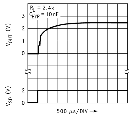
Figure 30. Turn-ON Waveform
