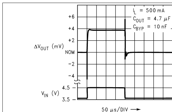
Figure 42. Line Transient Response
