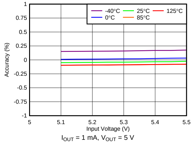
图 16. 5.0-V Accuracy vs V_{IN} (Line Regulation)
