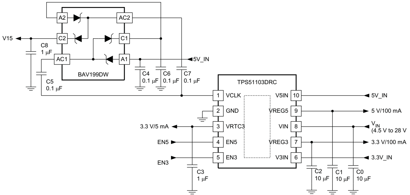
Figure 2. Typical Application
