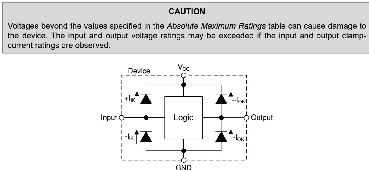
图 8-2. Electrical Placement of Clamping Diodes for Each Input and Output
