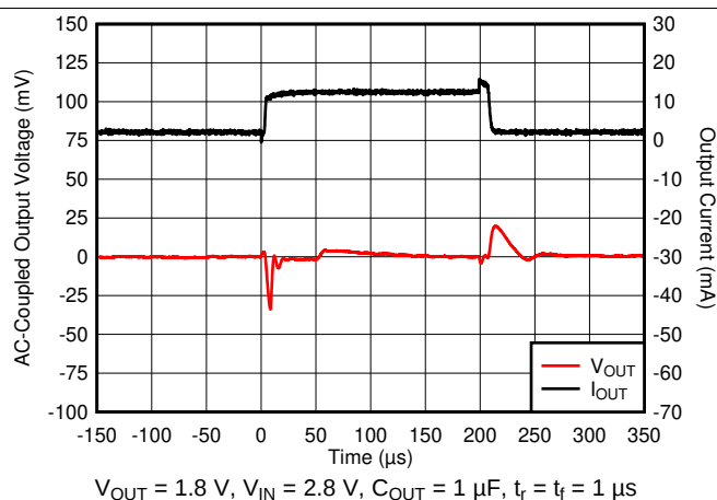
图 12. I_{OUT} Transient From 1\text{ mA} to 10\text{ mA}
