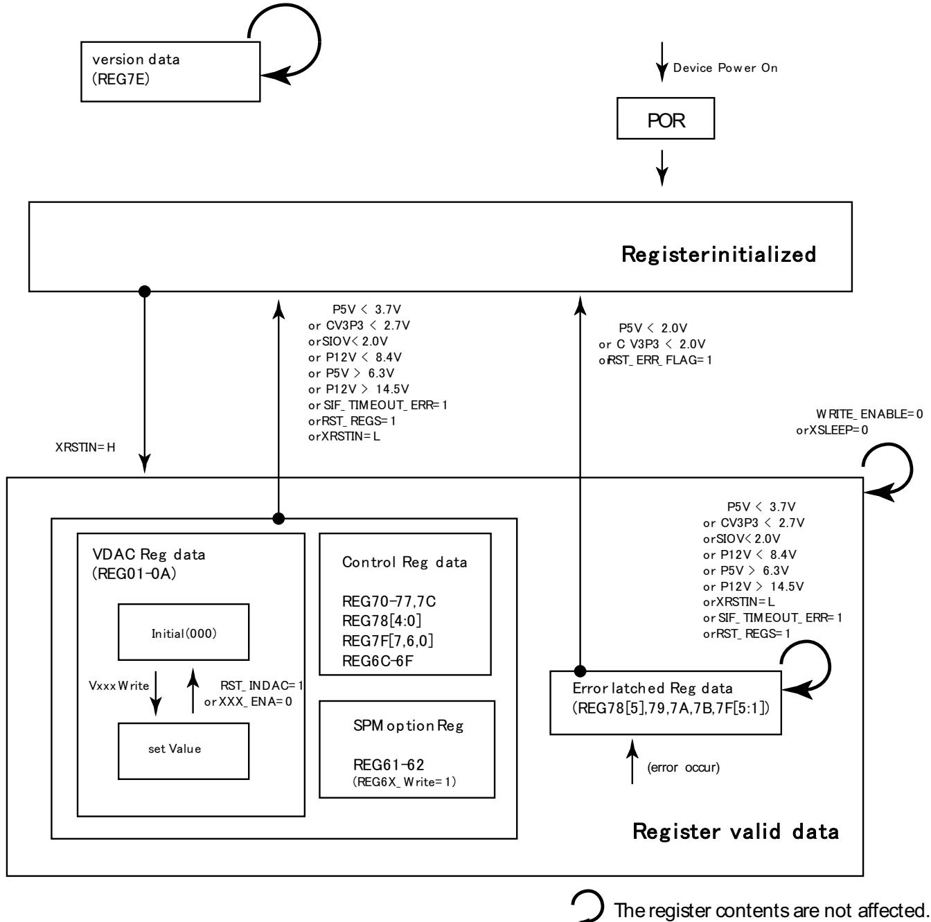
Figure 17. Register Behavior
