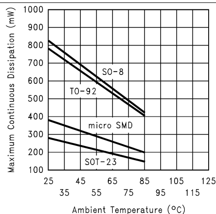
Figure 14. Thermal Information
