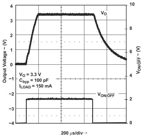
Figure 8-12. Turn-On Time
