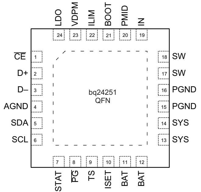
YFF Package / RGE Package 30-Pin DSBGA / 24-Pin QFN Top View / Top View
