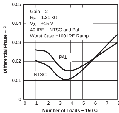
Figure 35. Differential Phase vs Number of Loads
