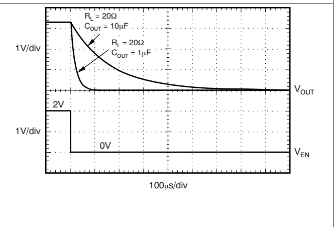
Figure 22. TPS73701 Turnoff Response
