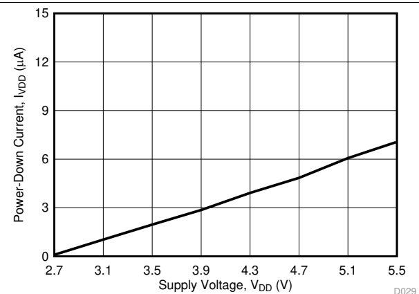
图 29. Supply Current vs Supply Voltage
