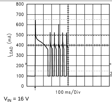
Figure 16. Short-Circuit Current
