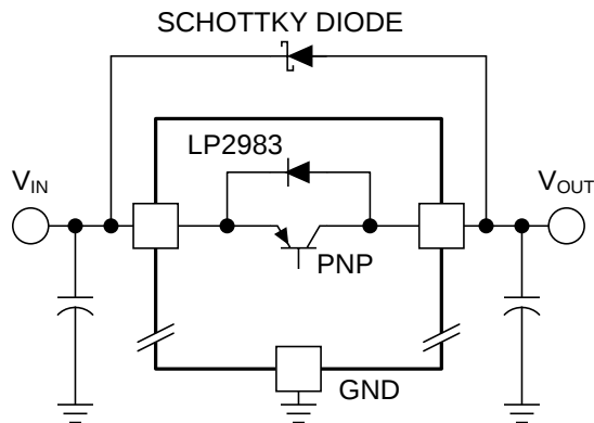
Figure 22. Adding External Schottky Diode Protection
