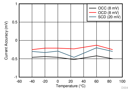
图 7-4. Overcurrent Accuracy Across Temperature
