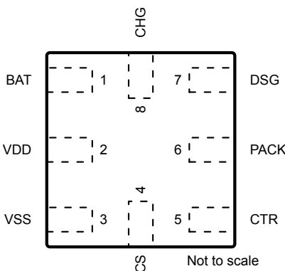
图 6-1. RUG Package 8-Pin X2QFN Top View
