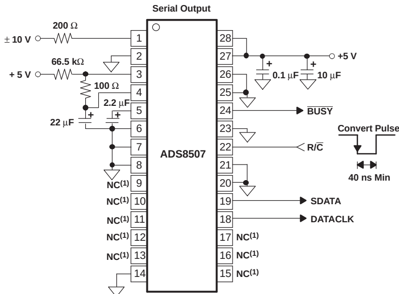
Figure 32. Basic \pm 10\text{-V} Operation With Serial Output
