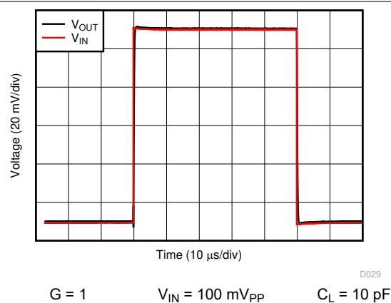
图 6-23. Small-Signal Step Response
