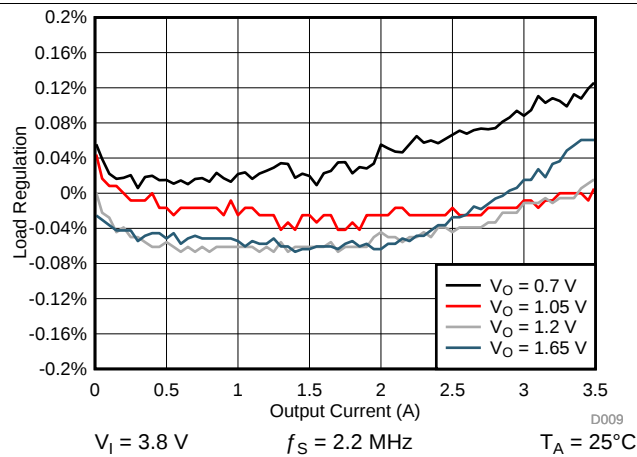
图 4-12. SMPS Load Regulation for SMPS1 and SMPS2 Single-Phase PWM Mode
