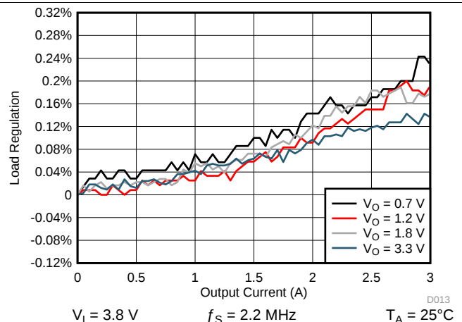
图 4-13. SMPS Load Regulation for SMPS3, PWM Mode
