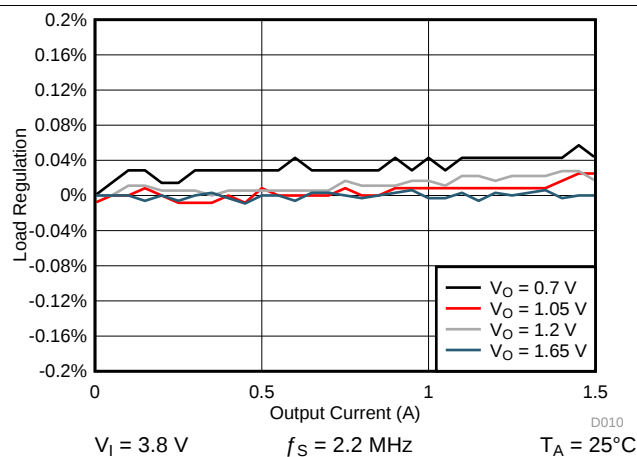
图 4-14. SMPS Load Regulation for SMPS4 in PWM Mode
