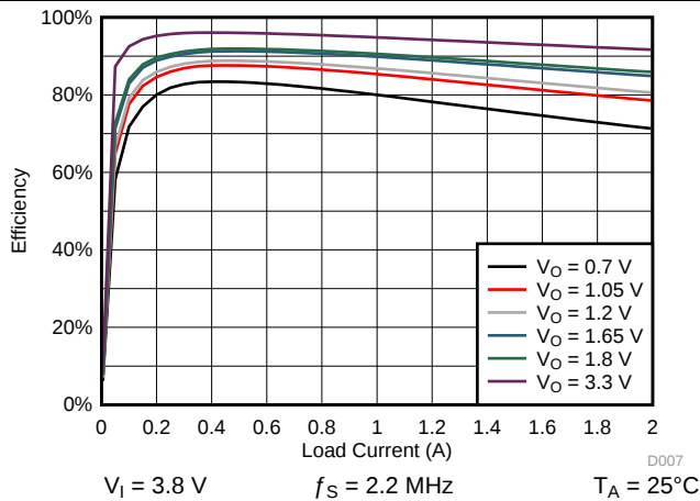
图 4-10. SMPS Efficiency for SMPS5 in PWM Mode
