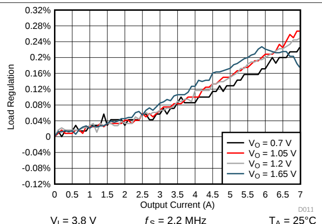
图 4-15. SMPS Load Regulation for SMPS12 in Dual-Phase PWM Mode
