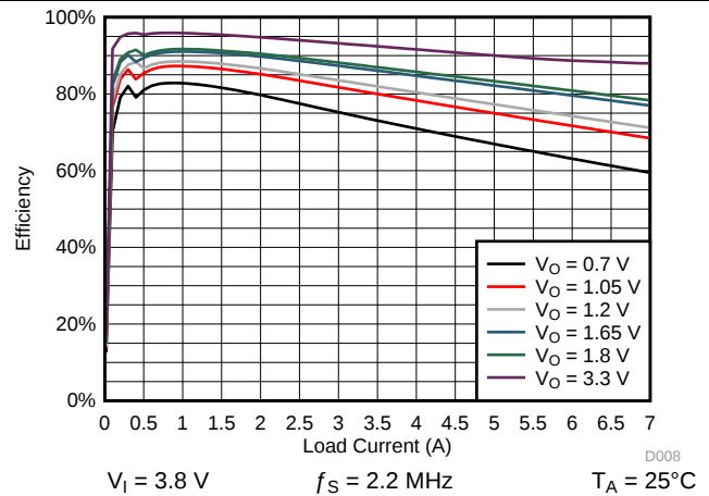
图 4-11. SMPS Efficiency for SMPS12 in Dual-Phase PWM Mode
