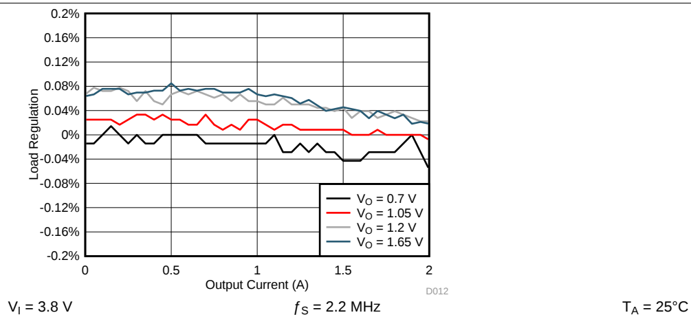
图 4-16. SMPS Load Regulation for SMPS5 in PWM Mode
