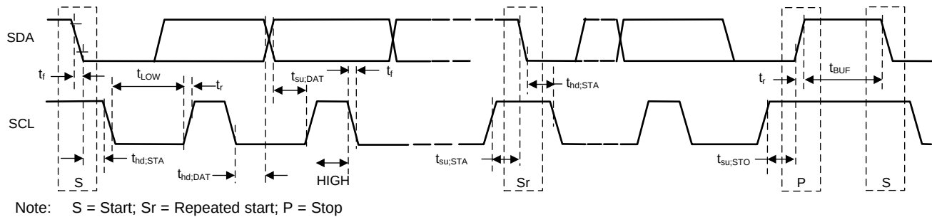
图 4-1. Serial Interface Timing Diagram For F/S Mode
