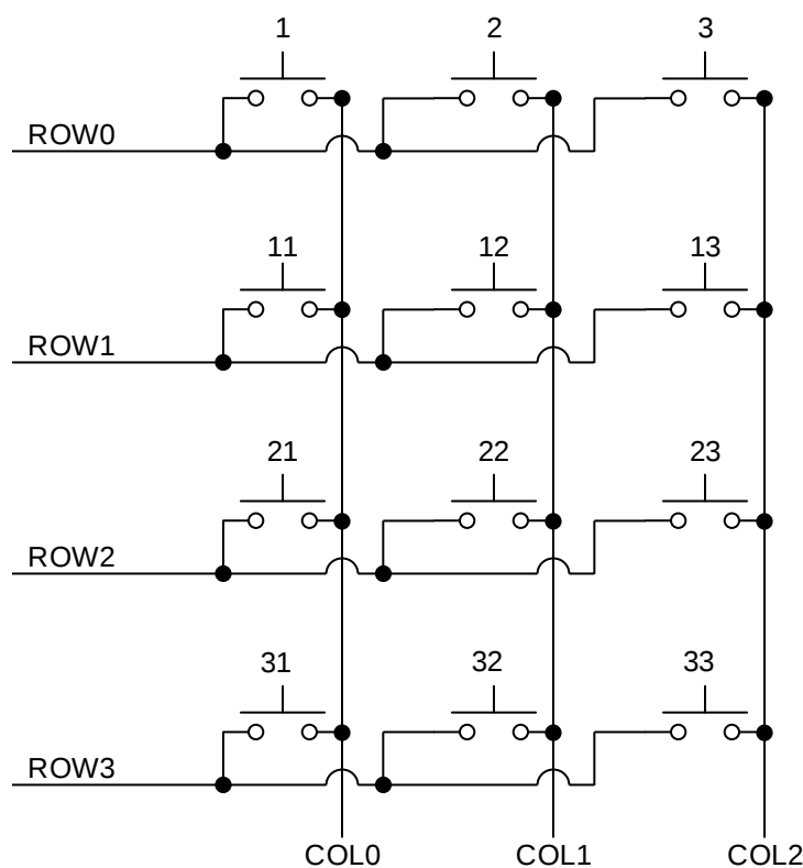
Figure 33. Keypad Schematic
