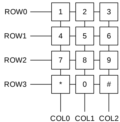
Figure 32. Example Keypad
