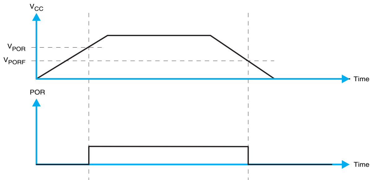
Figure 39. V_{POR}
