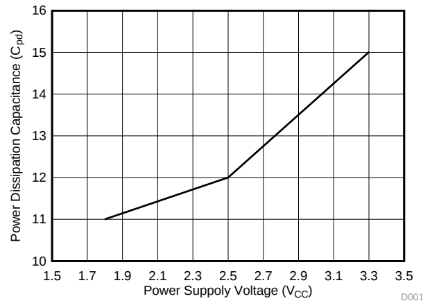
Figure 1. Power Dissipation Capacitance vs. Power Supply Voltage
