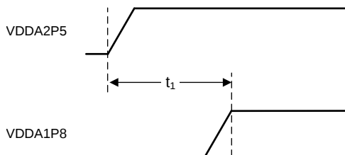
图 31. Three-Supply Mode Power Supply Sequence Diagram
