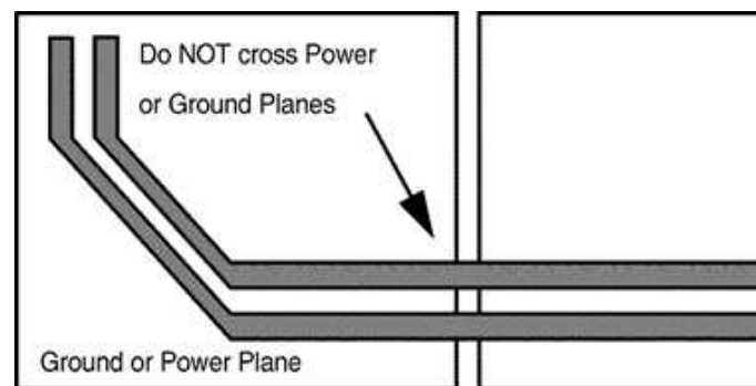
图 33. Differential Signal Pair-Plane Crossing
