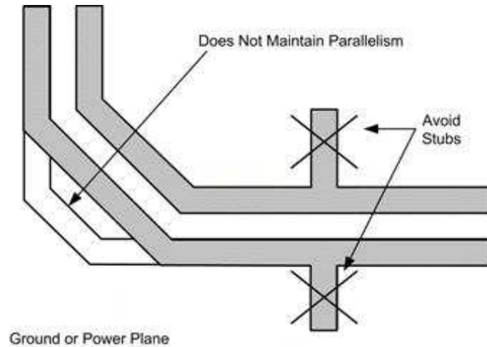
图 32. Avoiding Stubs in a Differential Signal Pair
