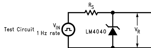
Figure 9. Test Circuit
