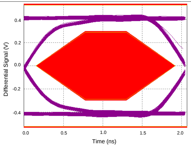
图 22. High Speed Eye Diagram Without TS5USBC41
