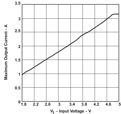
Figure 2. TPS61032 Maximum Output Current vs Input Voltage
