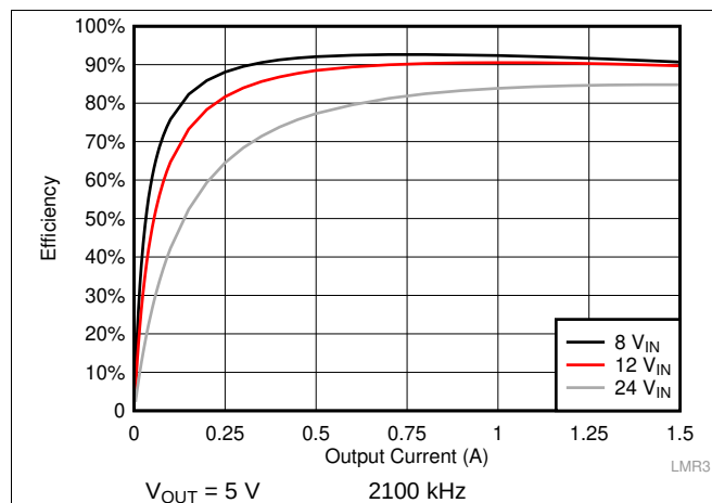
图 46. Efficiency
