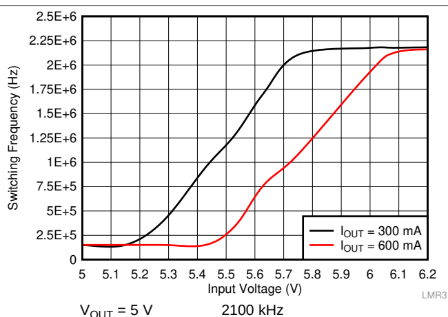
图 49. Frequency Dropout Characteristic
