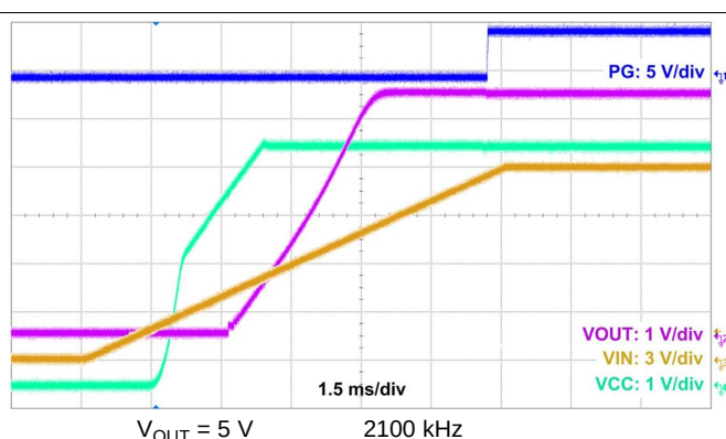
图 51. Start-Up Waveform
