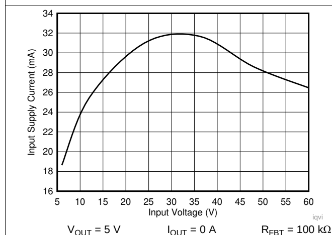
图 50. Input Supply Current
