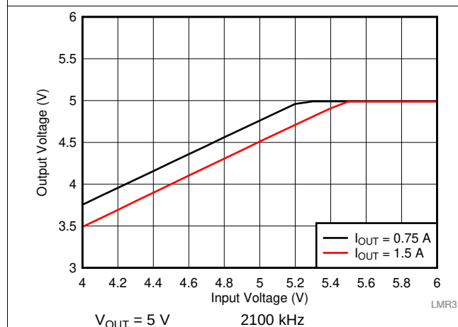
图 48. Overall Dropout Characteristic
