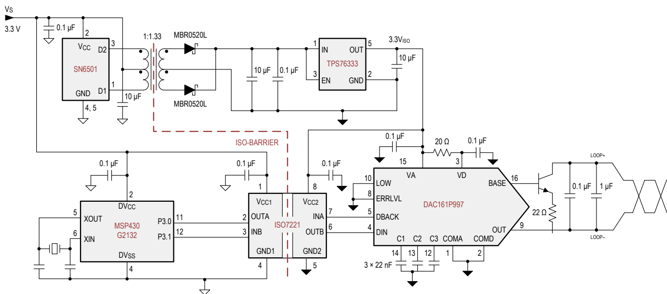
Figure 19. Isolated 4- to 20-mA Current Loop
