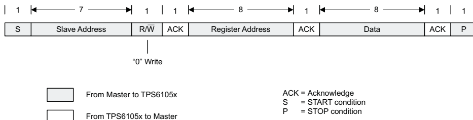
Figure 33. Write Data Transfer Format In F/S-Mode
