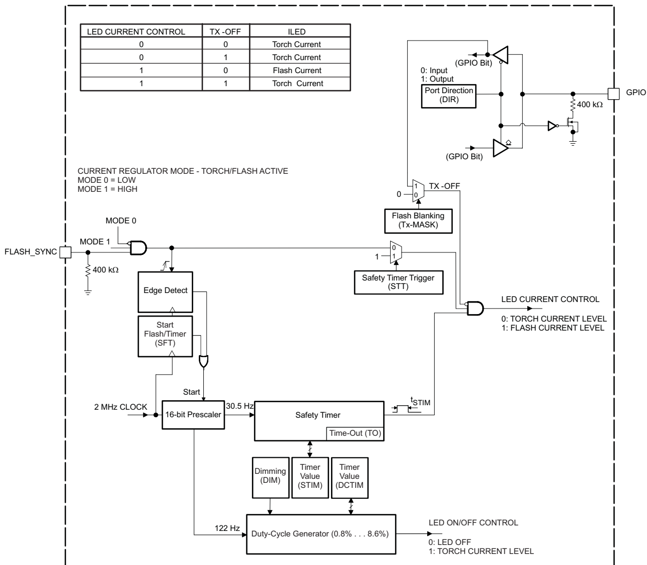
Figure 16. Timer Block Diagram (TPS61050)
