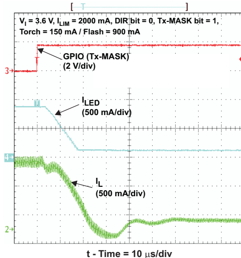
Figure 50. TX-Masking Operation
