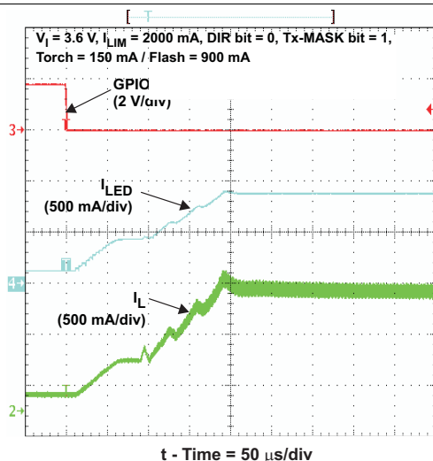
Figure 51. TX-Masking Operation
