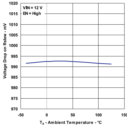
Figure 8. Voltage Drop ON Rslw for Current Reference (Slew Rate / Rslw)
