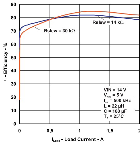
Figure 27. Efficiency vs Load Current for Different Rslw Resistors
