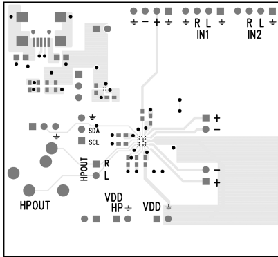
Figure 63. Top Layer
