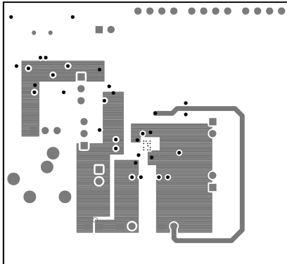
Figure 65. Layer 3
