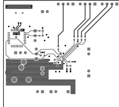
Figure 66. Bottom Layer
