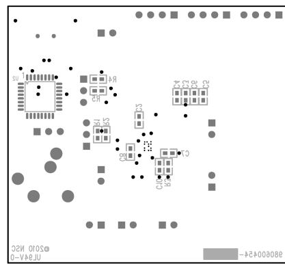
Figure 68. Bottom Silkscreen
