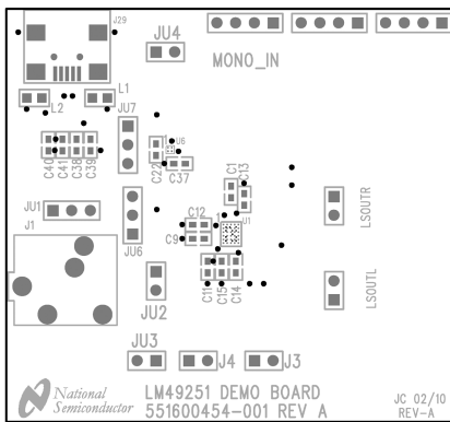
Figure 67. Top Silkscreen
