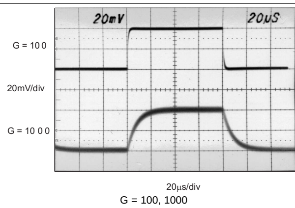
Figure 28. Small Signal
