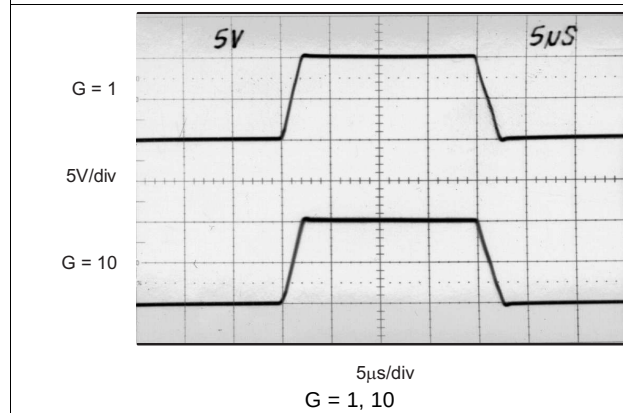
Figure 29. Large Signal
