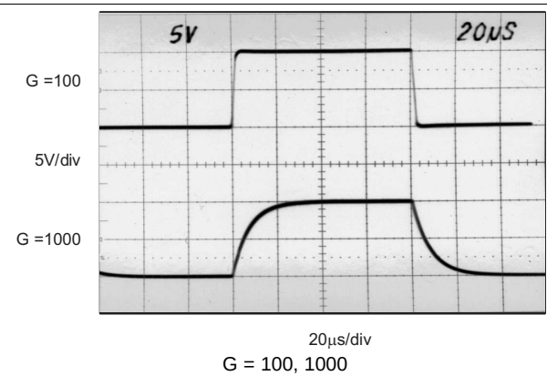
Figure 30. Large Signal
