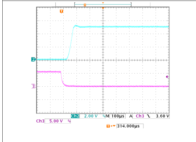
Figure 21. Enable Transient Response vs Time ( C_L = 1\ \mu\text{F} , I_L = 1\ \text{mA} )
