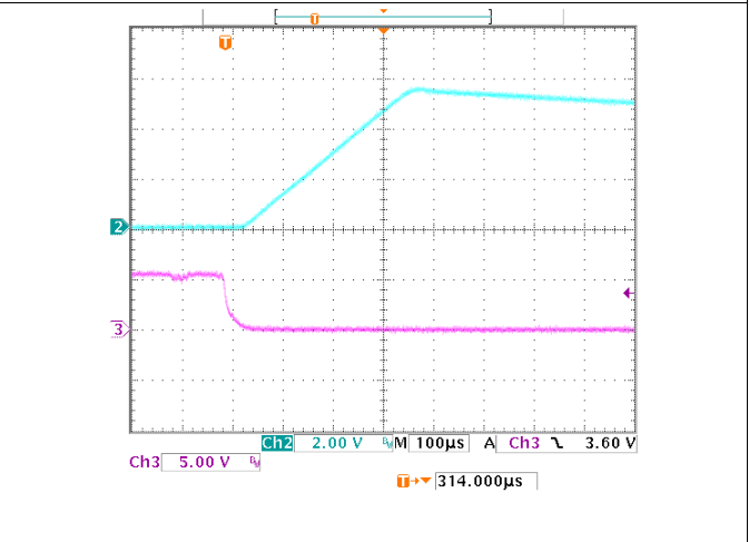
Figure 22. Enable Transient Response vs Time ( C_L = 10\ \mu\text{F} , I_L = 1\ \text{mA} )
