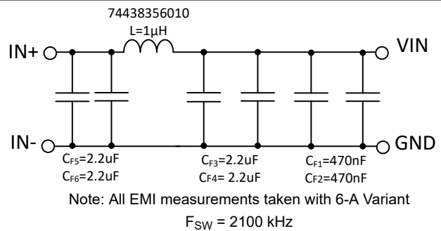
图 10-44. Recommended Input EMI Filter
