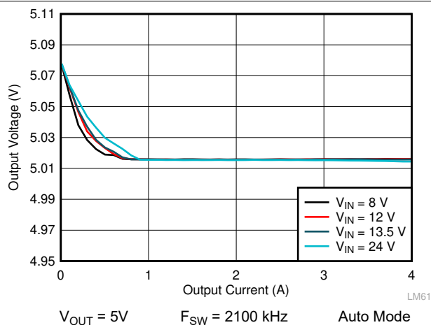
图 10-15. LM61440-Q1 Load and Line Regulation
