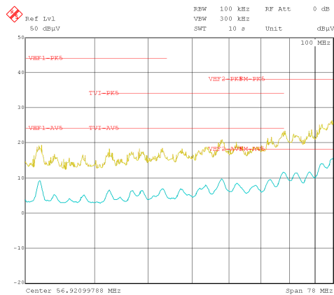
图 10-43. Conducted EMI versus CISPR25 Limits (Yellow: Peak Signal, Blue: Average Signal)
