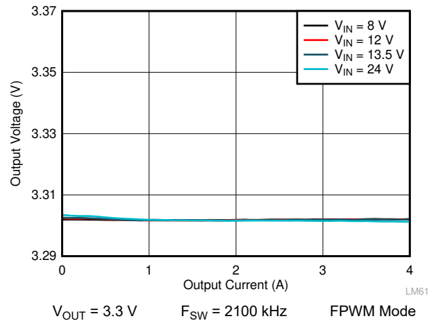
图 10-12. LM61440-Q1 Load and Line Regulation
