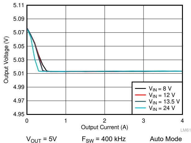
图 10-13. LM61440-Q1 Load and Line Regulation
