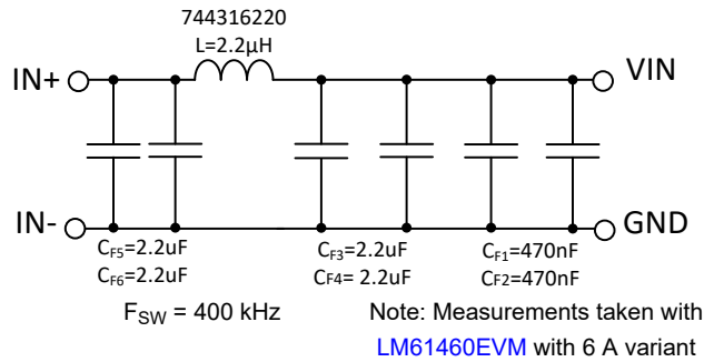
图 10-41. Recommended Input EMI Filter
