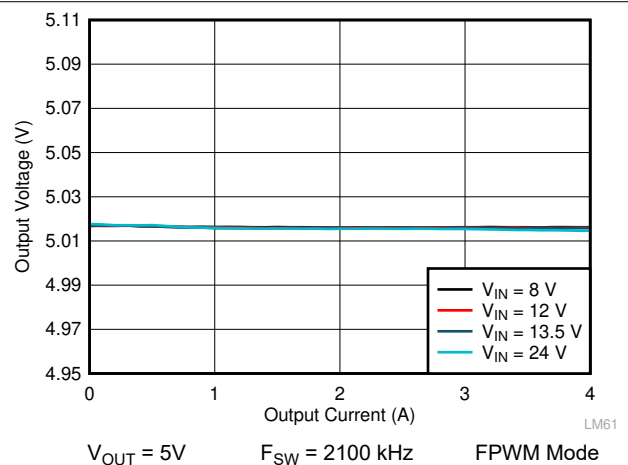
图 10-16. LM61440-Q1 Load and Line Regulation
