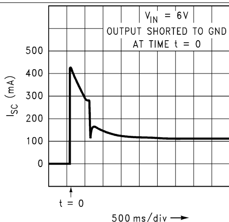
Figure 19. Short-Circuit Current
