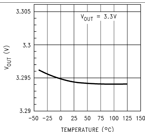
Figure 2. 3.3-V Output Voltage vs Temperature
