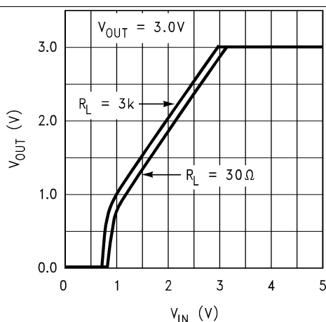
Figure 6. 3-V Dropout Characteristics
