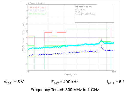
Figure 9-30. Radiated EMI Log Vertical versus CISPR25 Limits
