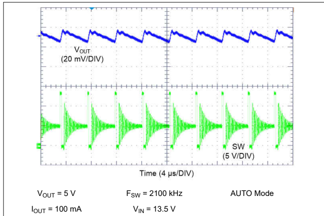
Figure 9-17. LM62435-Q1 Switching Waveform and V_{OUT} Ripple
