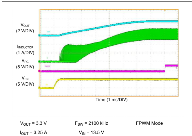
Figure 9-19. LM62435-Q1 Start-up with 3.25 A
