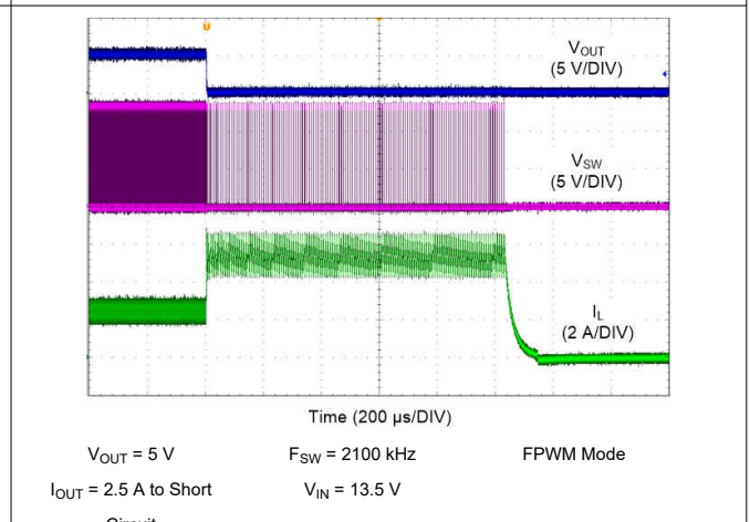
Figure 9-20. LM62435-Q1 Short Circuit Protection
