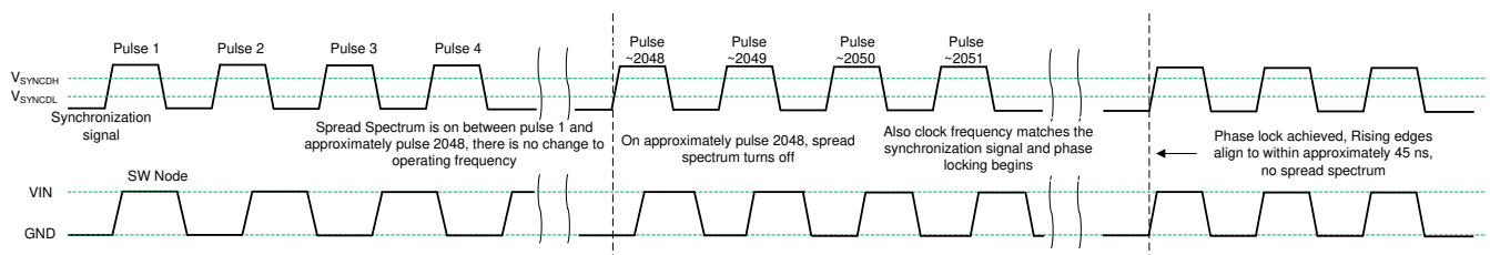
Figure 8-12. Synchronization Process
