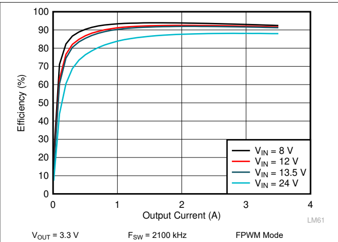
Figure 9-6. LM62435-Q1 Efficiency
