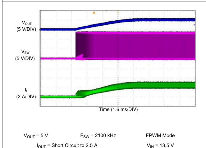
Figure 9-21. LM62435-Q1 Short Circuit Recovery
