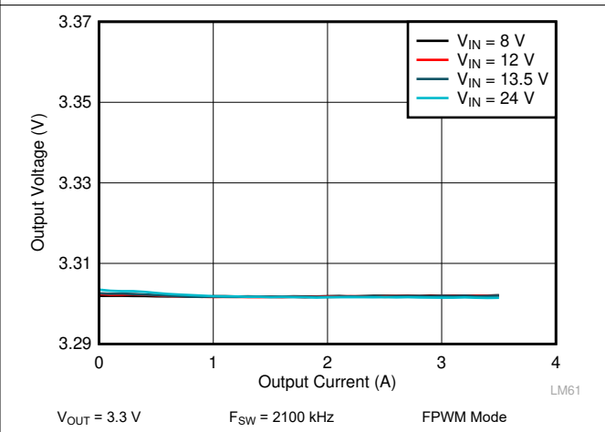
Figure 9-10. LM62435-Q1 Load and Line Regulation
