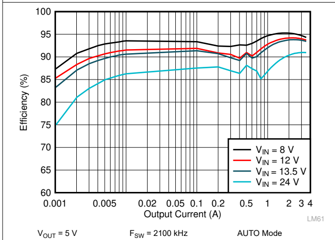
Figure 9-7. LM62435-Q1 Efficiency
