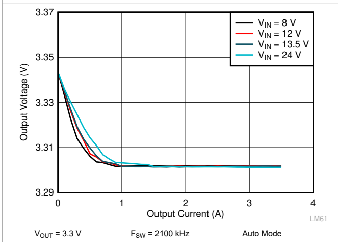
Figure 9-9. LM62435-Q1 Load and Line Regulation
