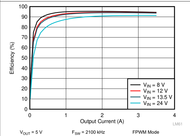
Figure 9-8. LM62435-Q1 Efficiency
