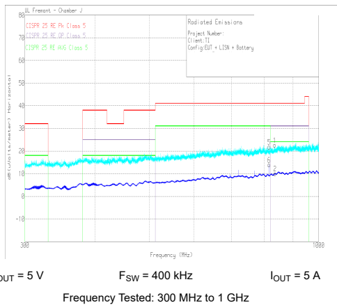
Figure 9-31. Radiated EMI Log Horizontal versus CISPR25 Limits
