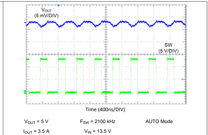
Figure 9-18. LM62435-Q1 Switching Waveform and V_{OUT} Ripple
