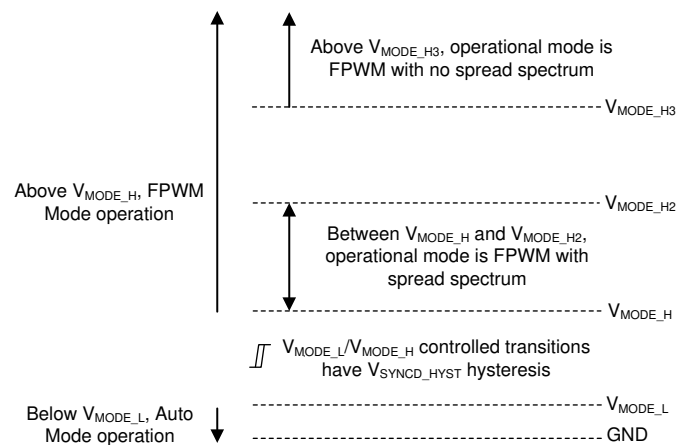
Figure 8-2. Level-Dependent Mode Selection Settings
