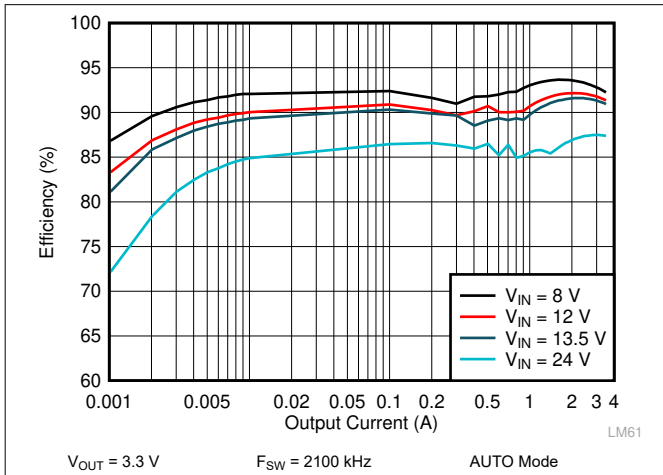
Figure 9-5. LM62435-Q1 Efficiency
