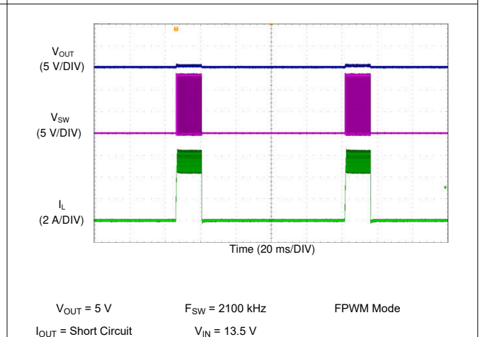
Figure 9-22. LM62435-Q1 Short Circuit Performance
