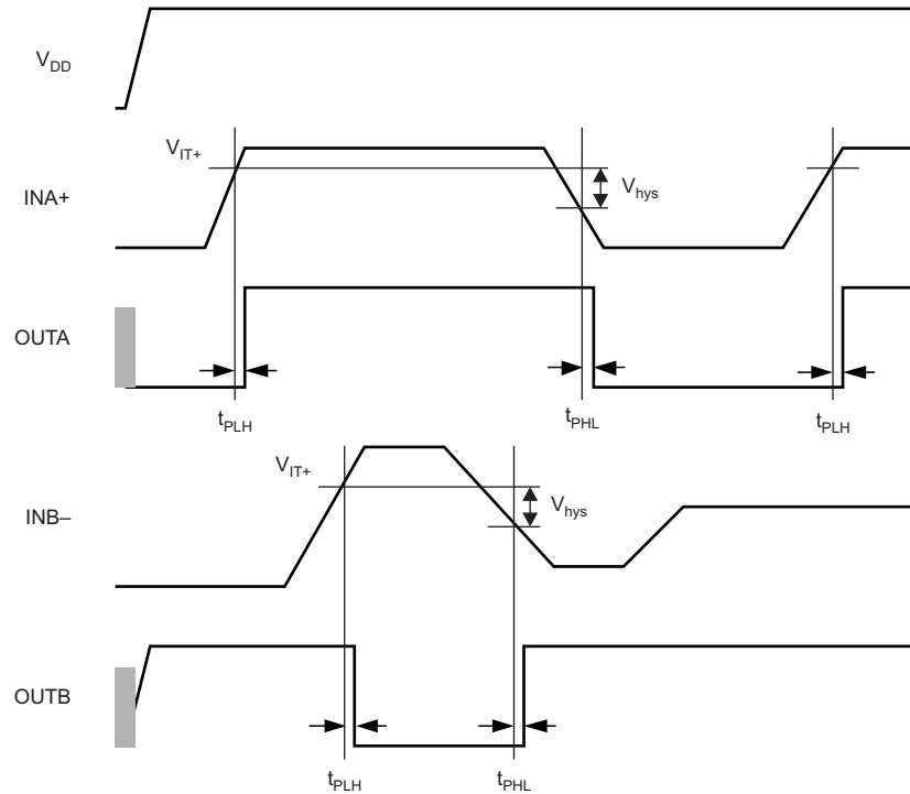
Figure 1. Timing Diagram
