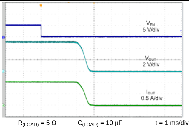
Figure 19. Turnoff Response
