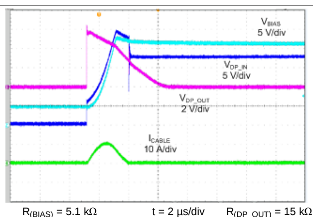
Figure 53. Enabled, DP_IN Shorted to Battery
