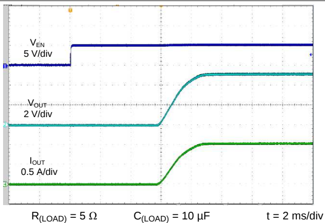
Figure 18. Turnon Response
