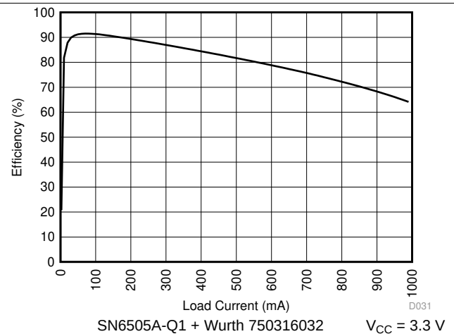
图 6. Efficiency vs Load Current
