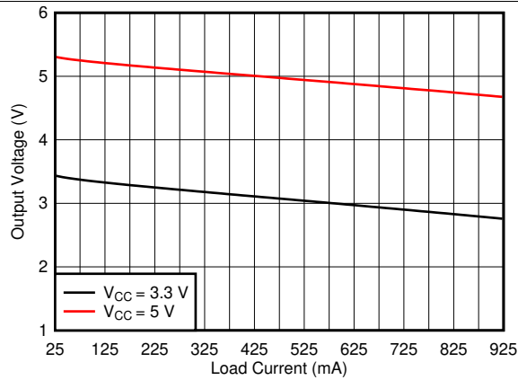
图 1. Output Voltage vs Load Current
