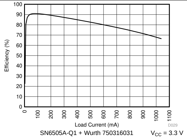
图 4. Efficiency vs Load Current
