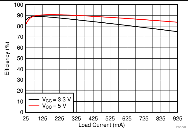
图 2. Efficiency vs Load Current
