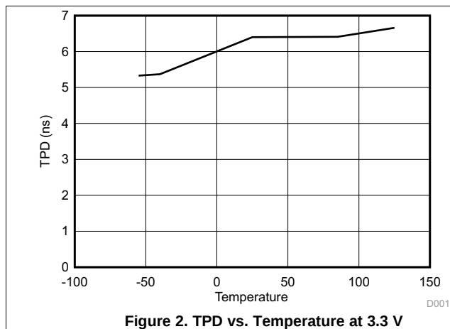
Figure 2. TPD vs. Temperature at 3.3 V
