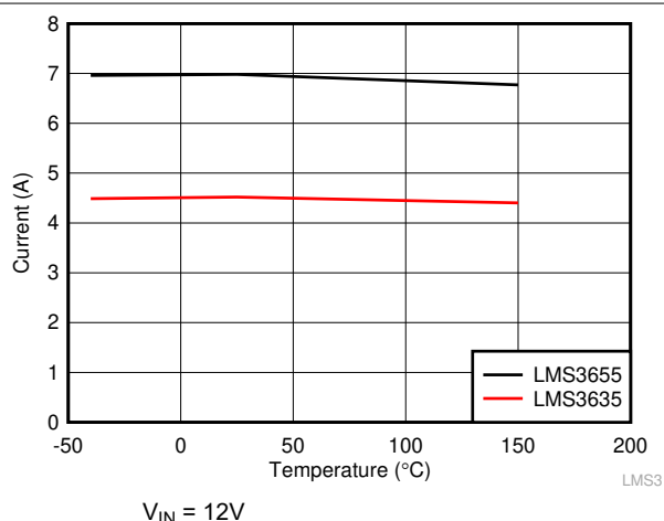
图 7-4. Low-Side/Valley Current Limit for LMS36x5-Q1
