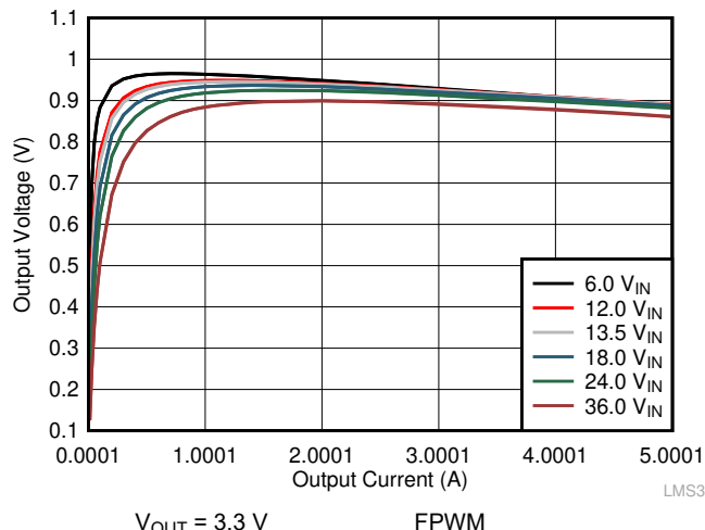
图 9-18. Efficiency
