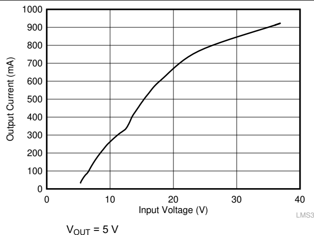
图 9-9. Load Current for PFM-to-PWM Transition
