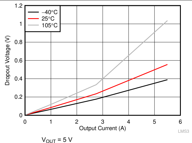
图 9-10. Dropout for - 3% Regulation
