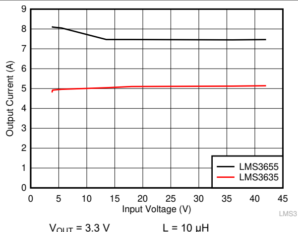
图 9-26. Output Current Level for Overcurrent Protection Trip
