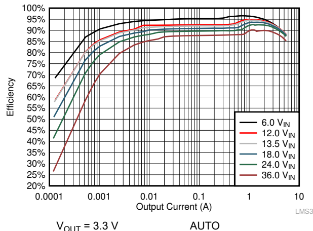
图 9-17. Efficiency
