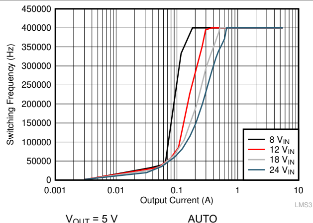
图 9-12. Switching Frequency vs Load Current
