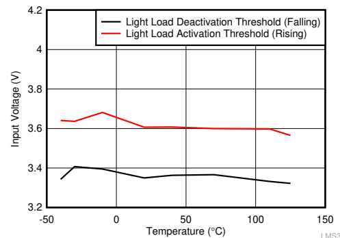
图 8-8. Input Voltage for Mode Change — 3.3-V Output, 10-µH Inductor
