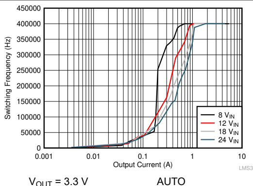
图 9-25. Switching Frequency vs Load Current
