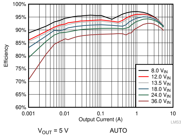
图 9-5. Efficiency
