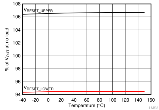
图 7-8. RESET Threshold as Percentage of Output Voltage
