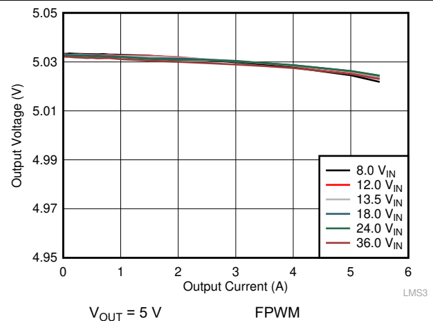
图 9-8. Load and Line Regulation
