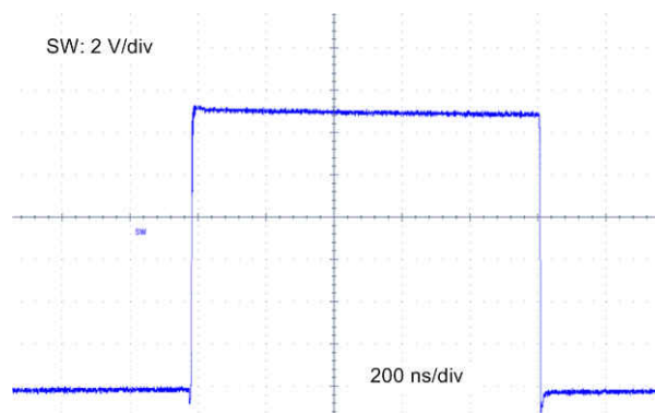
图 8-1. Switch Node Waveform ( V_{IN} = 13.5\text{ V} , I_{OUT} = 5.5\text{ A} )
