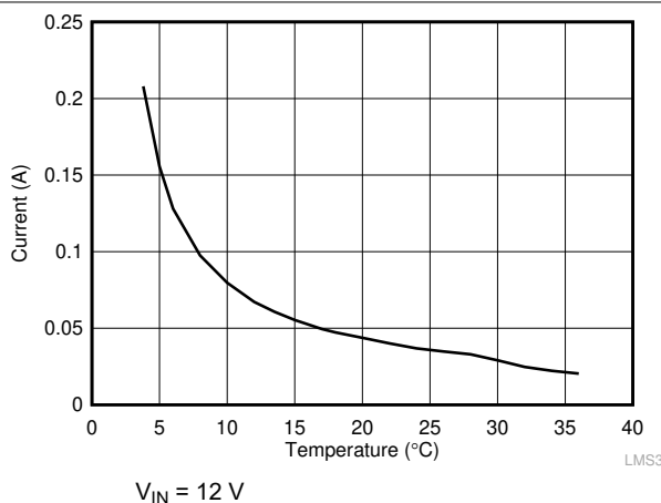
图 7-5. Short Circuit Average Input Current for LMS3635-Q1
