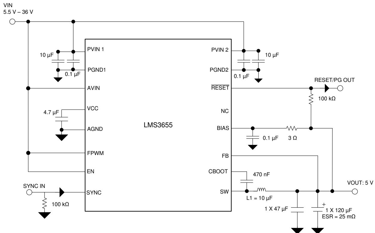
图 9-4. Fixed 5-V, 5.5-A Output Power Supply
