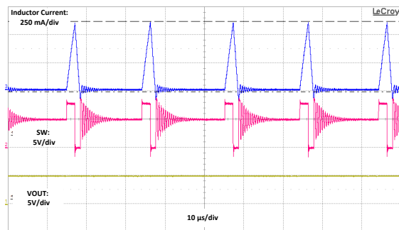
图 8-7. Typical PFM Switching Waveforms
