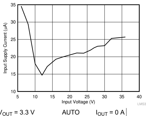
图 9-21. Input Supply Current (Includes Leakage Current of Capacitor)
