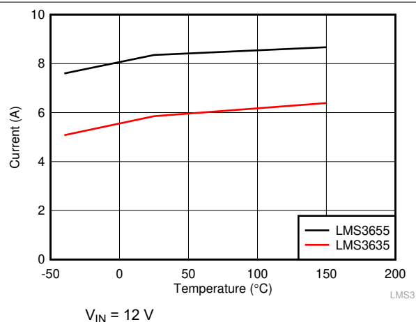
图 7-3. High-Side/Peak Current Limit for LMS36x5-Q1
