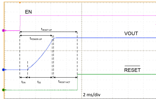
图 8-4. Typical Start-Up Waveform
