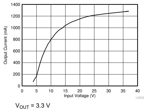
图 9-22. Load Current for PFM-to-PWM Transition
