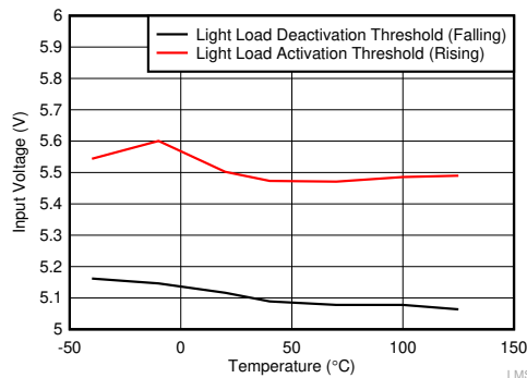
图 8-9. Input Voltage for Mode Change — 5-V Output, 10-µH Inductor
