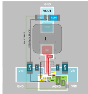
图 11-2. Recommended Layout for LMS36x5-Q1
