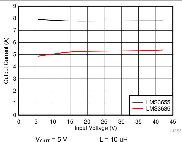
图 9-13. Output Current Level Limit Before Overcurrent Protection
