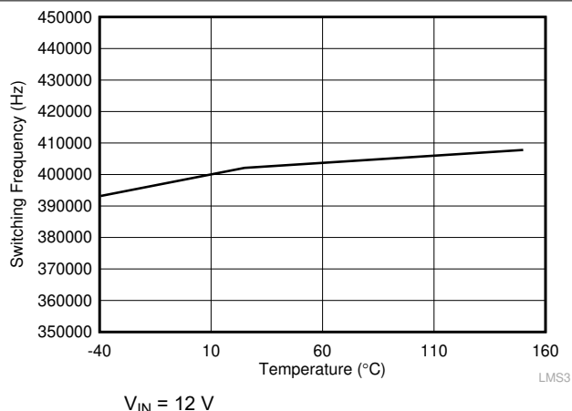
图 7-2. Switching Frequency vs Temperature
