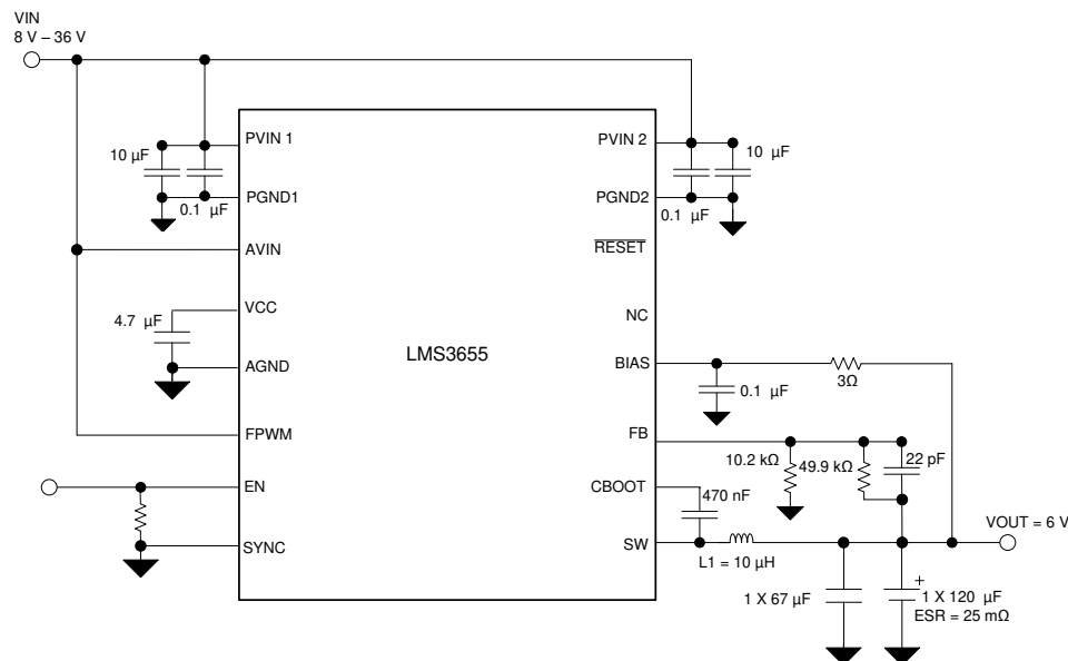
图 9-30. 6-V Output Power Supply
