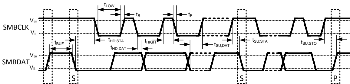
Figure 2. SMBus Communication
