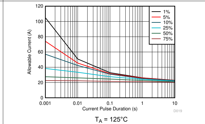
图 8-9. Maximum Repetitive Pulsed Current vs. Pulse Duration
