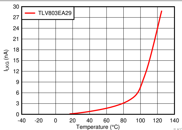
图 9. Leakage Current Over Temperature for TLV803EA29
