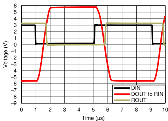
图 9-2. 250 kbit/s Driver to Receiver Loopback Timing Waveform, V_{CC} = 3.3 \text{ V}
