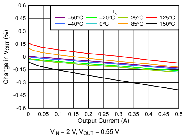
图 6-17. 0.55-V Load Regulation vs I_{OUT}
