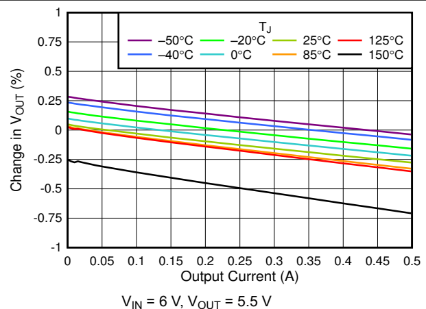
图 6-18. 5.5-V Load Regulation vs I_{OUT}
