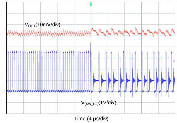
图 91. Transient from PWM-to-PFM Mode (2-Phase Output)
