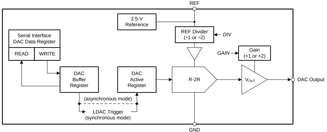
Figure 57. DACx0504 DAC Block Diagram
