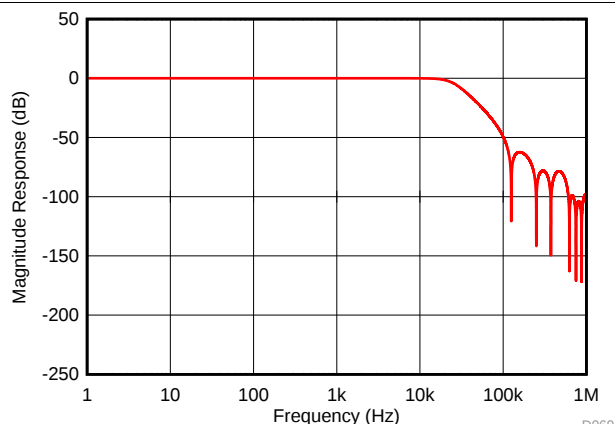
图 79. Digital Filter Response for OSR = 4
