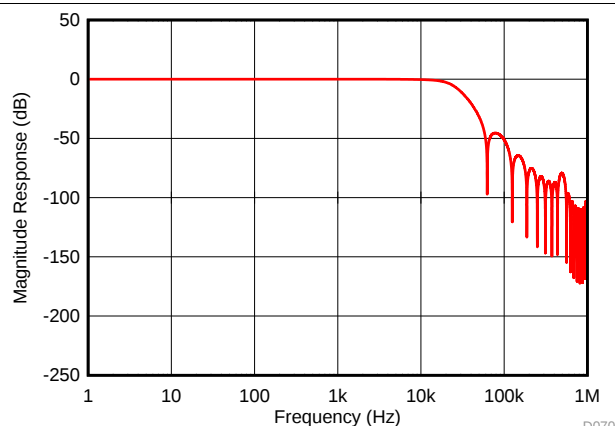
图 78. Digital Filter Response for OSR = 2
