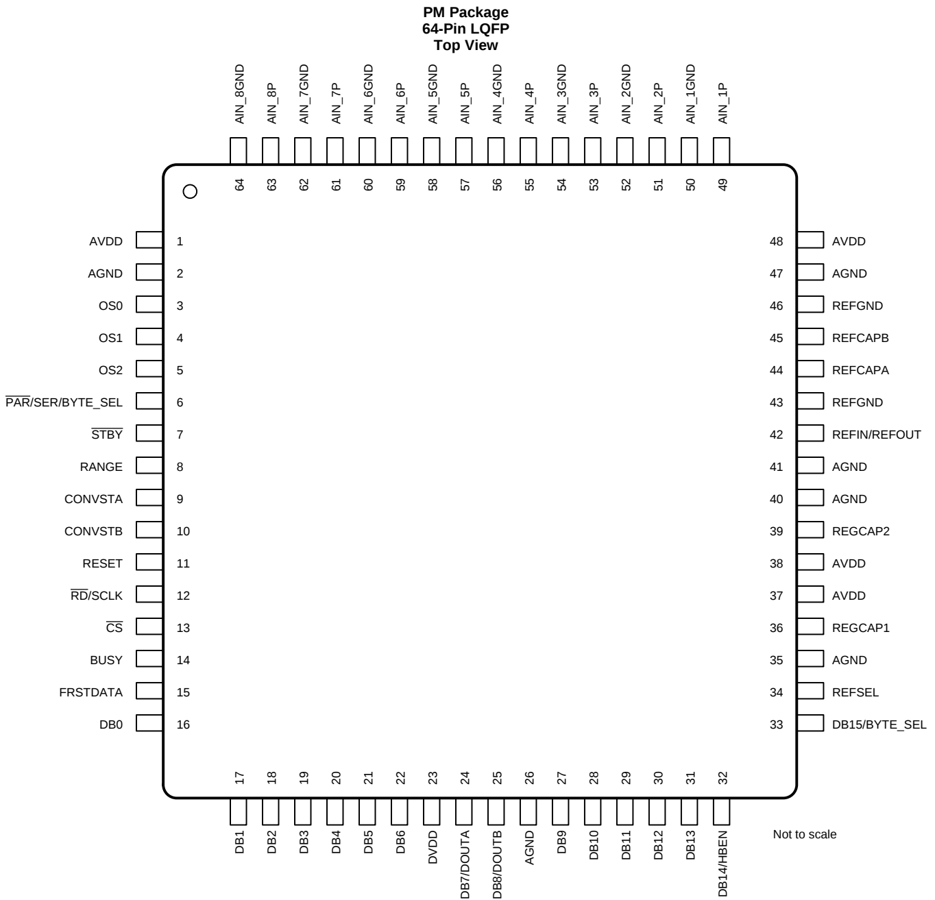
Pin Functions
