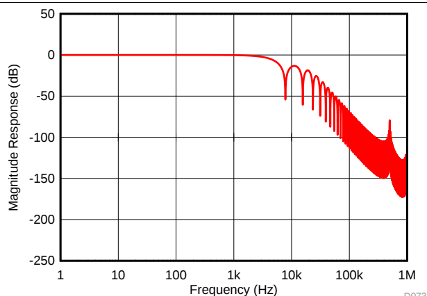
图 81. Digital Filter Response for OSR = 16
