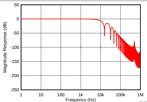
图 80. Digital Filter Response for OSR = 8
