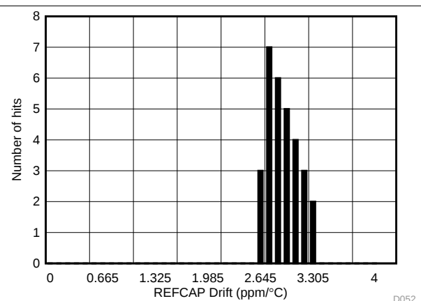
图 63. Reference Buffer Temperature Drift Histogram
