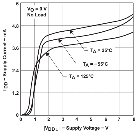
Figure 37. TLC2274-Q1 Supply Current vs Supply Voltage
