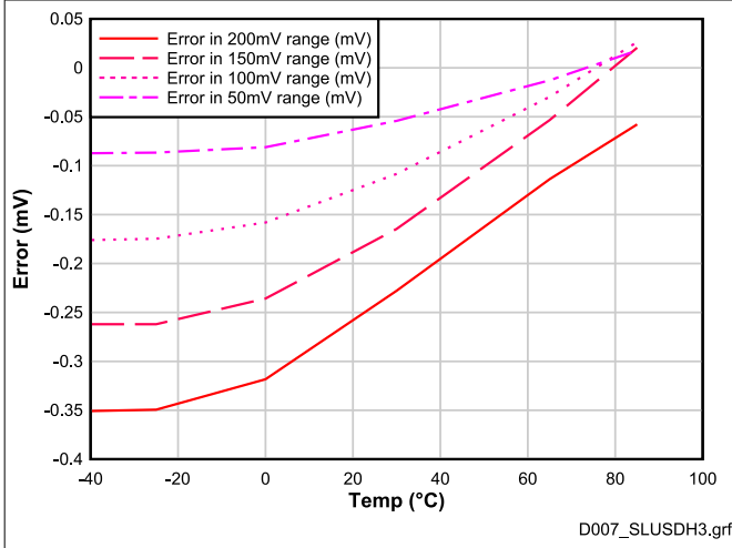
图 7-10. Current Measurement Error vs. Temperature
