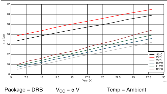
图 7-11. Sleep Mode Current Across V_{SUP} and Temperature
