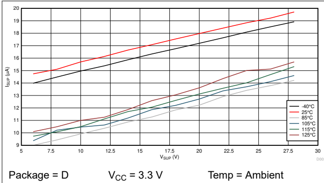
图 7-7. Sleep Mode Current Across V_{SUP} and Temperature
