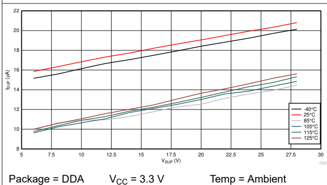
图 7-9. Sleep Mode Current Across V_{SUP} and Temperature
